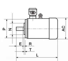
IMV1
