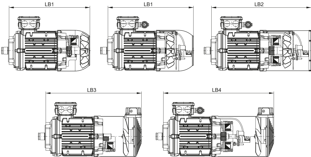
Description of the dimensions L, LB, LB0,... see page 384
